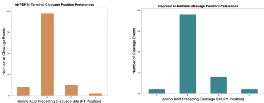
Figure 4. N-terminal Cleavage Position Preferences of Neprosin and ANPEP
