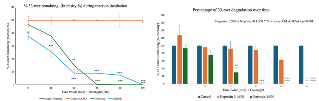
Figure 1. Degradation of 33-mer peptide by Neprosin and ANPEP over time
