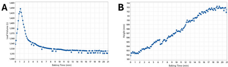
Figure 2. Evolution of bread loaf dimensions during baking.
