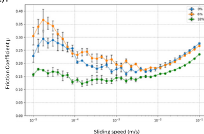
Fig. Stribeck curve for Formulations 0%, 6%, and 10%
