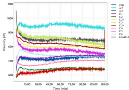
Figure 4. SC screening viscosity comparison at premix stage
