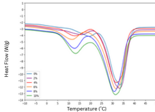
Fig. Melting curves of the six chocolate formulations
