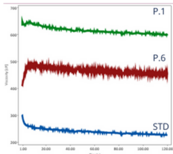
Figure 5. PP screening viscosity comparison at premix stage
