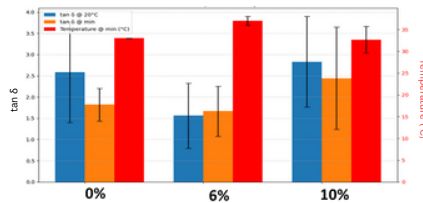
Fig. Comparison of \tan \delta values at 20°C and at their minima, and temperature at minima
