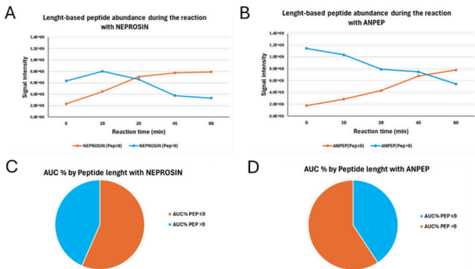
Figure 3. Abundance of peptides by length formed during the reaction with Neprosin (A) or ANPEP (B), and percentage of the area under the curve (AUC) corresponding to peptides identified
