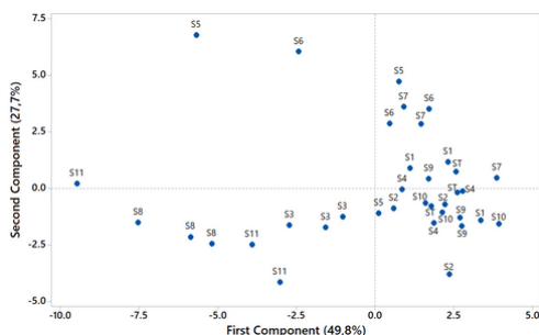
Figure 5. PCA score plot (convection oven tests).
