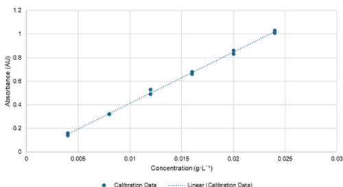
Figure 2. Calibration curve of PVOH solutions
