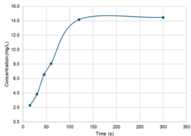
Figure 3. PVOH Dissolution During the First 300 Seconds of Immersion
