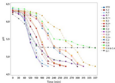
Figure 3. SC screening- fermentation curve
