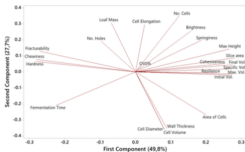
Figure 4. PCA loading plot (convection oven tests).
